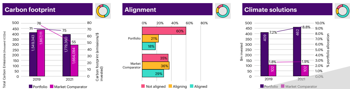
Figure 2: Example portfolio
